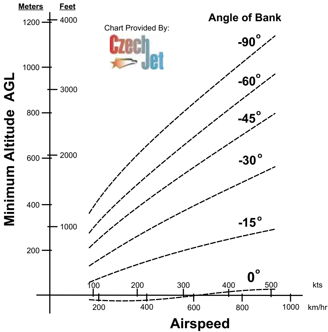
SINGLE SEAT - Minimum Height vs. Aircraft bank angle
