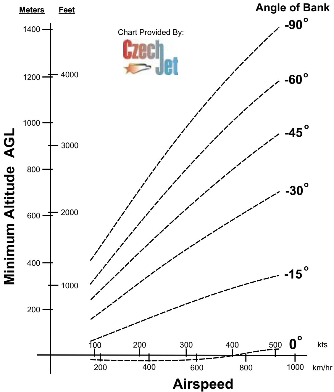
TWO SEAT - Minimum Height vs. Aircraft bank angle
